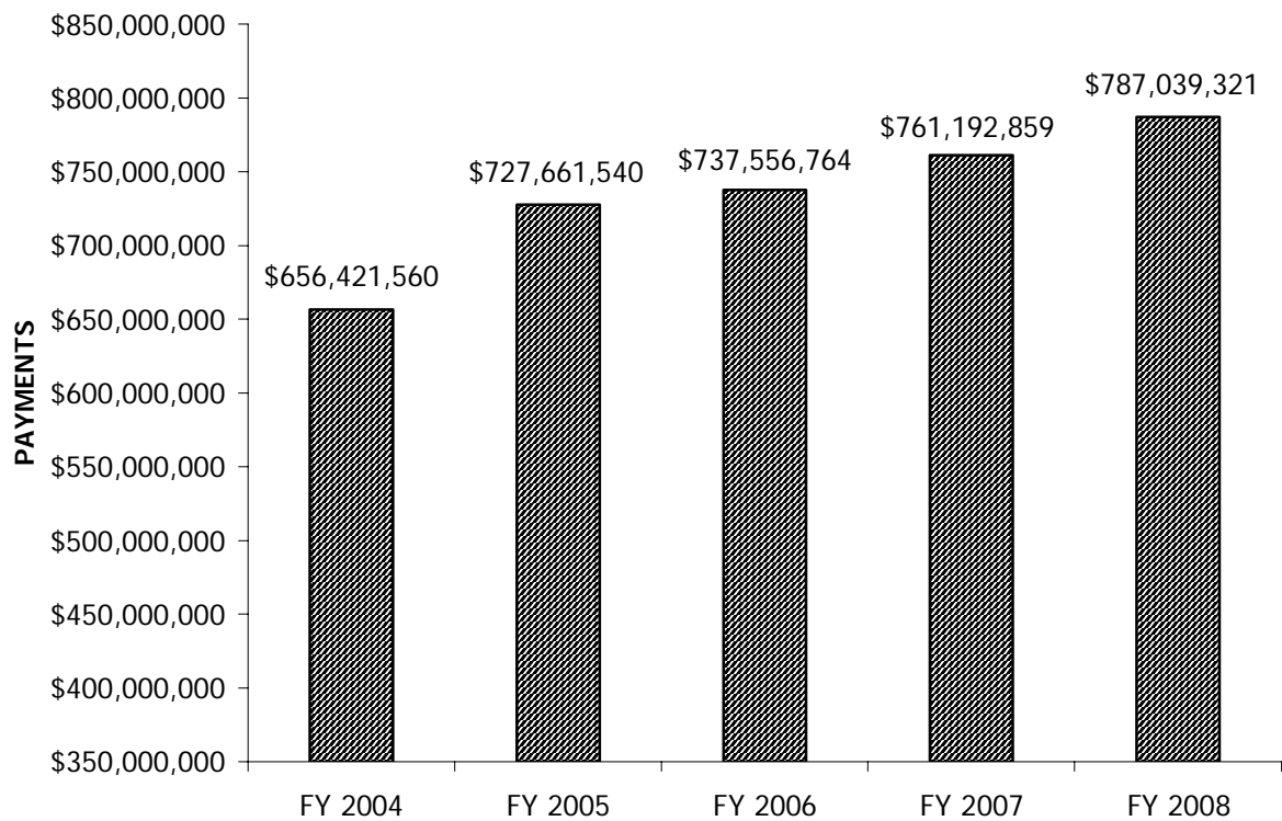
Figure 6. Food Stamps Annual Benefits Issued Fiscal Years 2004 - 2008
